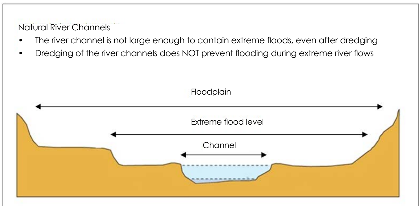
Figure 2: Natural river channels
