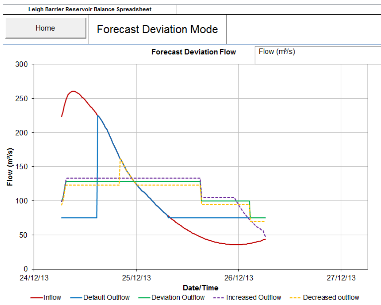
Figure 4.9: Discharge plots from the RBS for the hypothetical optimal strategy
